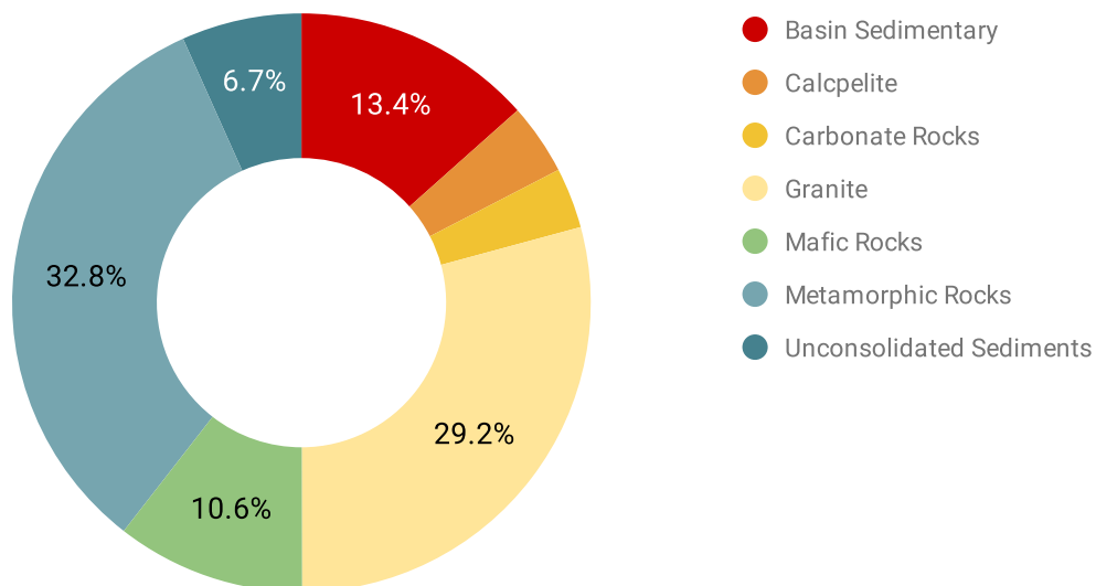
Figure II-5: Bedrock lithology by total surface area (source: MassGIS, BuroHappold Analysis)
